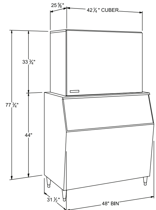
GB1060 on a B950 Bin. Stores 950 lbs. of ice, based on 35 lbs./cu.ft. at 90% of bin volume.
